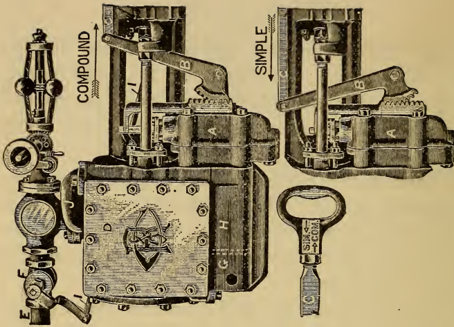
FIG. 34.—THE REEVES GOVERNOR AND VALVE GEAR FOR CHANGING FROM A SIMPLE TO A COMPOUND ENGINE.
